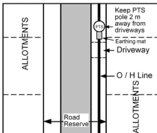
Figure 7: Positioning of earthed poles
