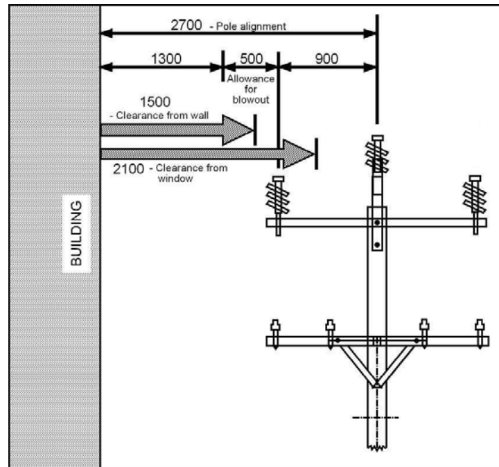
Figure 5 Compliance with ENA C(b)1
