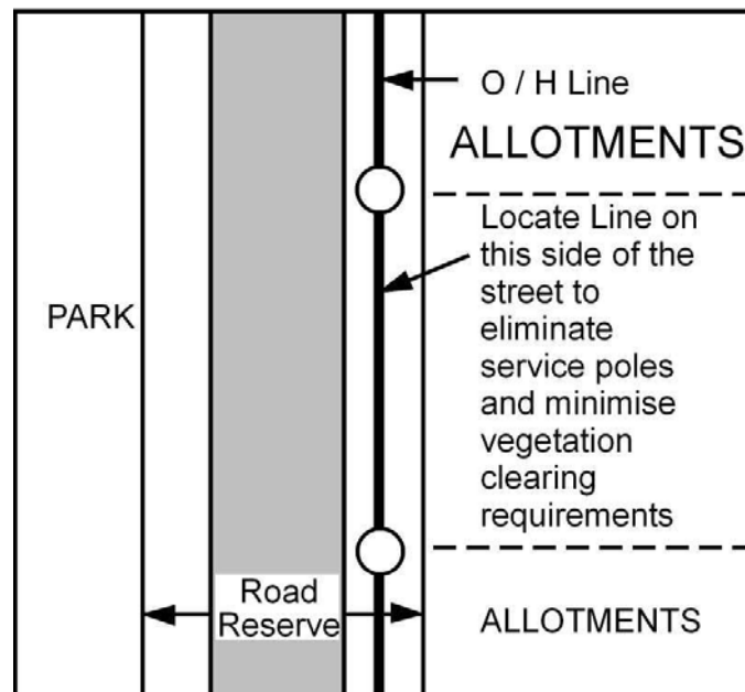
Figure 2: The advantage of careful pole positioning
