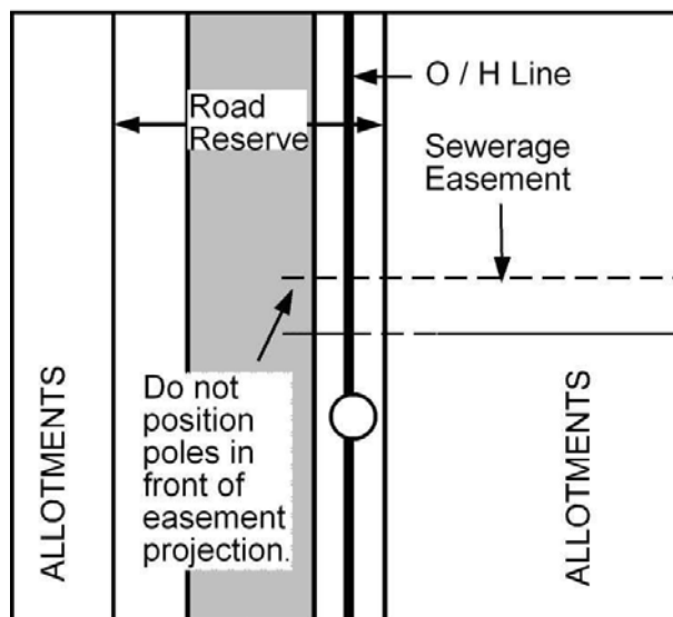
Figure 12: Poles within easements
