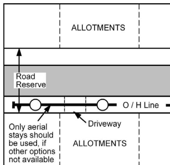
Figure 6: Location of stay poles
