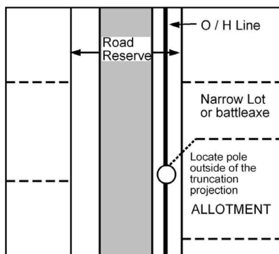
Figure 9: Location of poles on common lot boundaries
