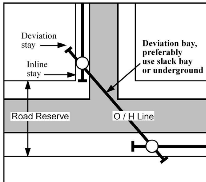
Figure 3: Deviation angles
