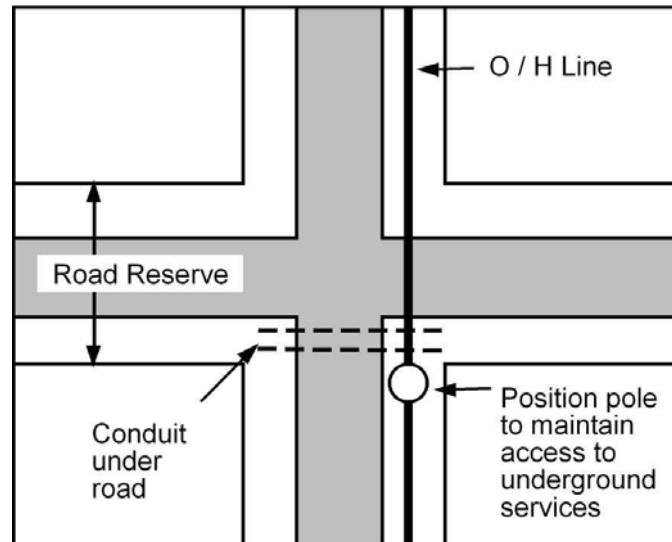
Figure 10: Proximity to underground services
