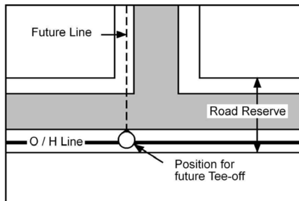
Figure 1: Consideration of future requirements
