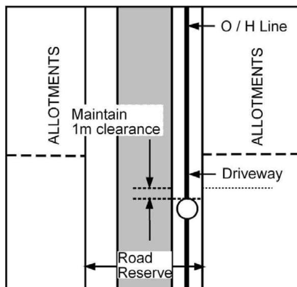
Figure 8: Poles near driveway crossovers
