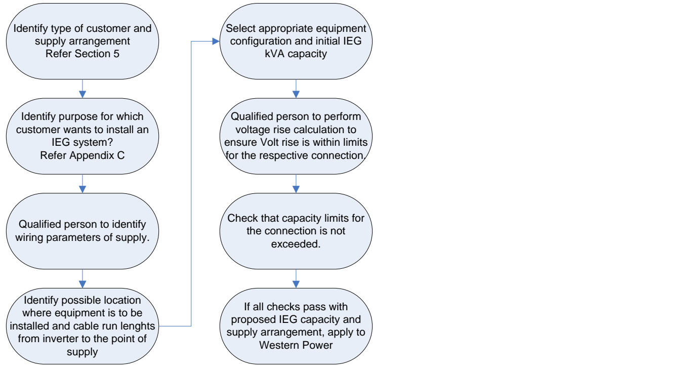
Figure 5: Basic assessment steps for an IEG connection
