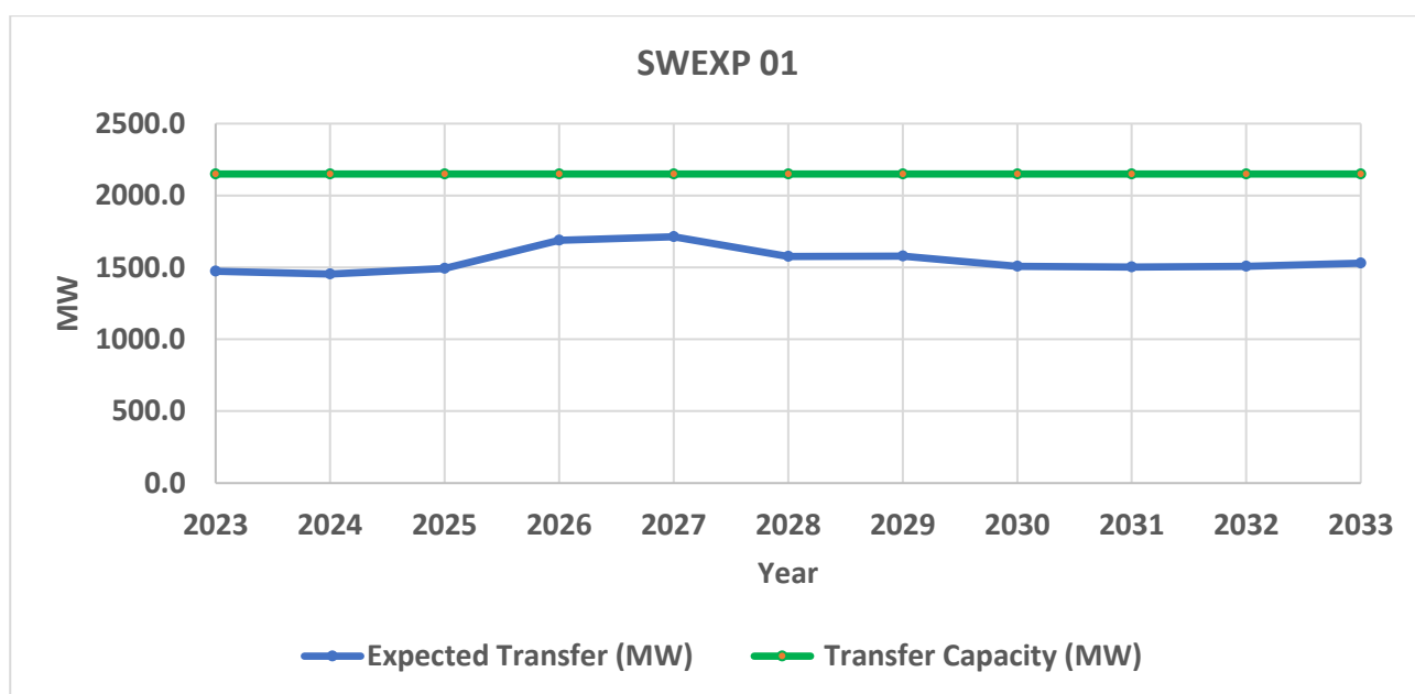
Figure 33: Expected transfer and transfer capacity in SWEXP 01 boundary – peak demand
