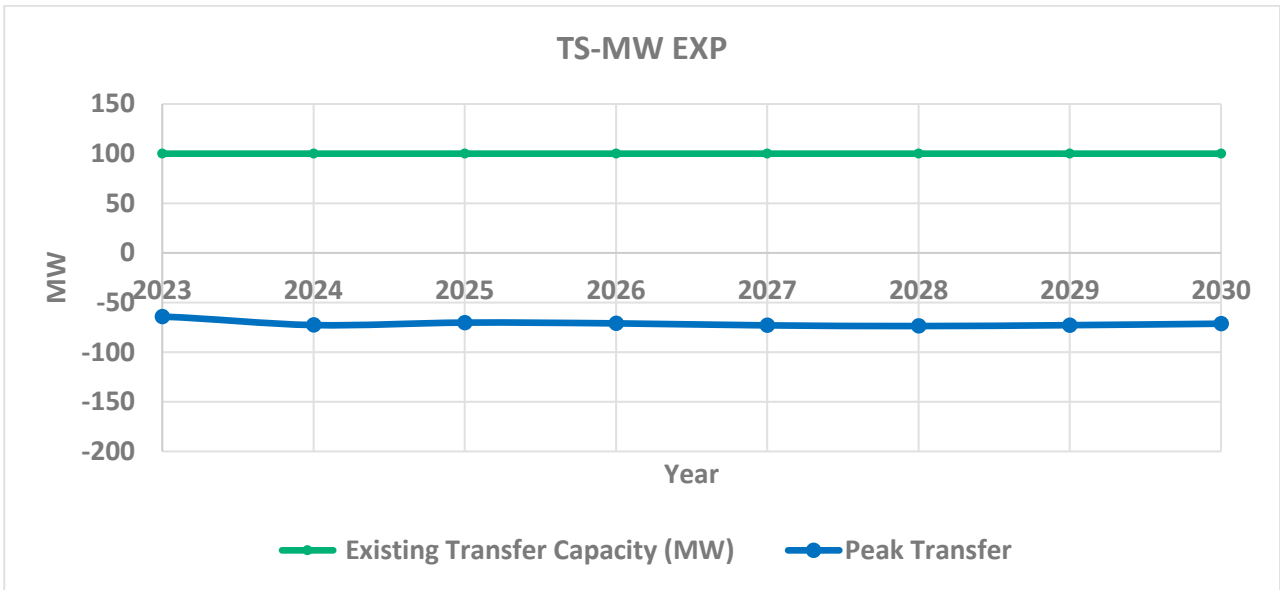
Figure 22: Expected transfer and transfer capacity in TS-MW EXP – peak demand
