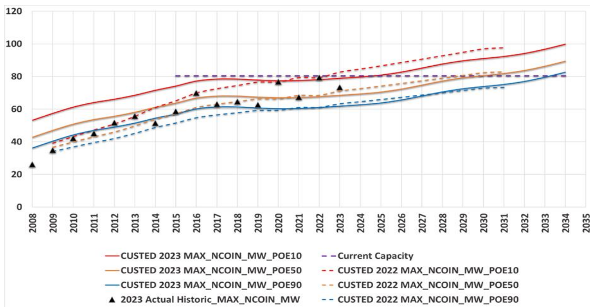
Figure 11: Waikiki non-coincidental historical and forecast maximum demand
