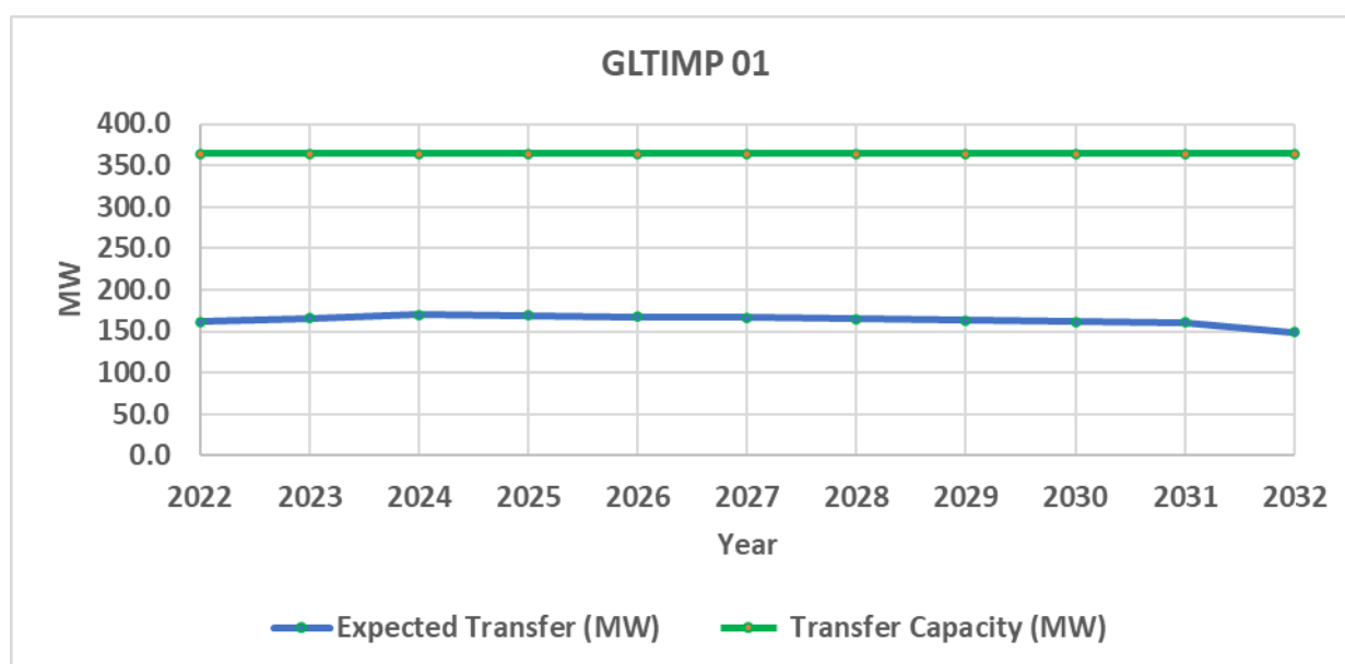
Figure 48: Expected transfer and transfer capacity in GLTIMP 01 boundary – peak demand
