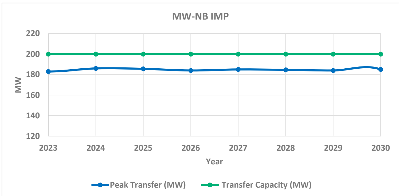
Figure 18: Expected transfer and transfer capacity in MW-NB IMP boundary – peak demand
