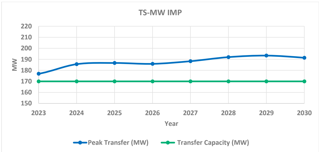
Figure 17: Expected transfer and transfer capacity in TS-MW IMP boundary – peak demand
