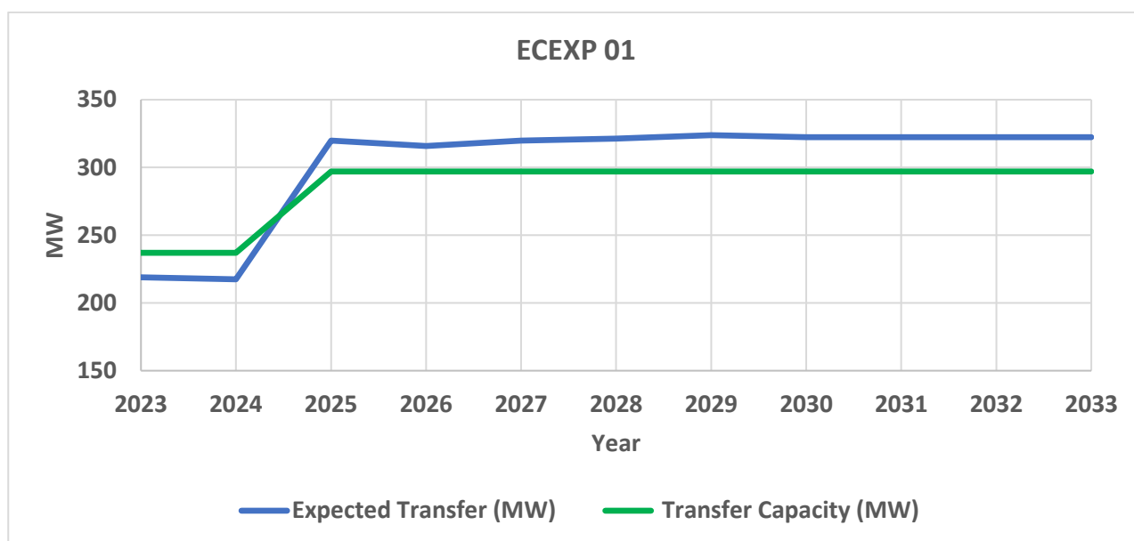
Figure 41: Expected transfer and transfer capacity in ECEXP 01 boundary – peak demand
