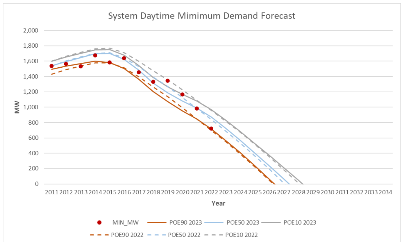
Figure 12: Historical and forecast system minimum demand - 2011 and 2034
