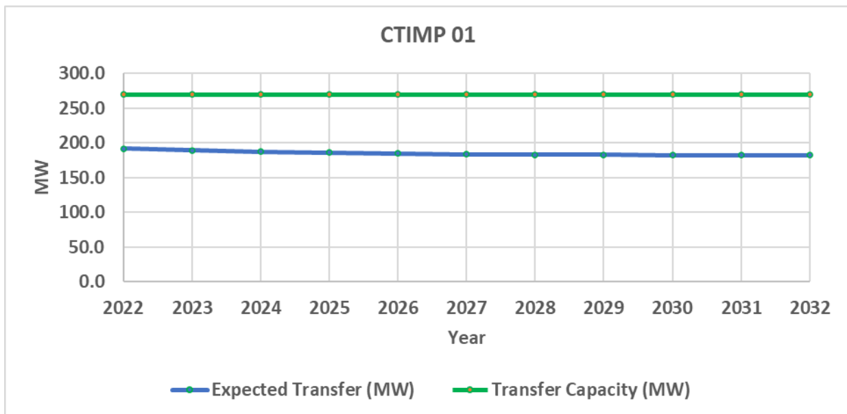
Figure 56: Expected transfer and transfer capacity in CTIMP 01 boundary – peak demand
