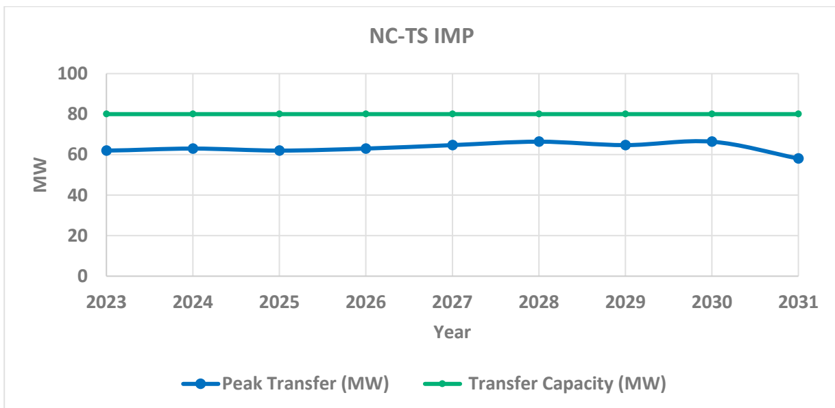
Figure 16: Expected transfer and transfer capacity in NC-TS IMP boundary – peak demand
