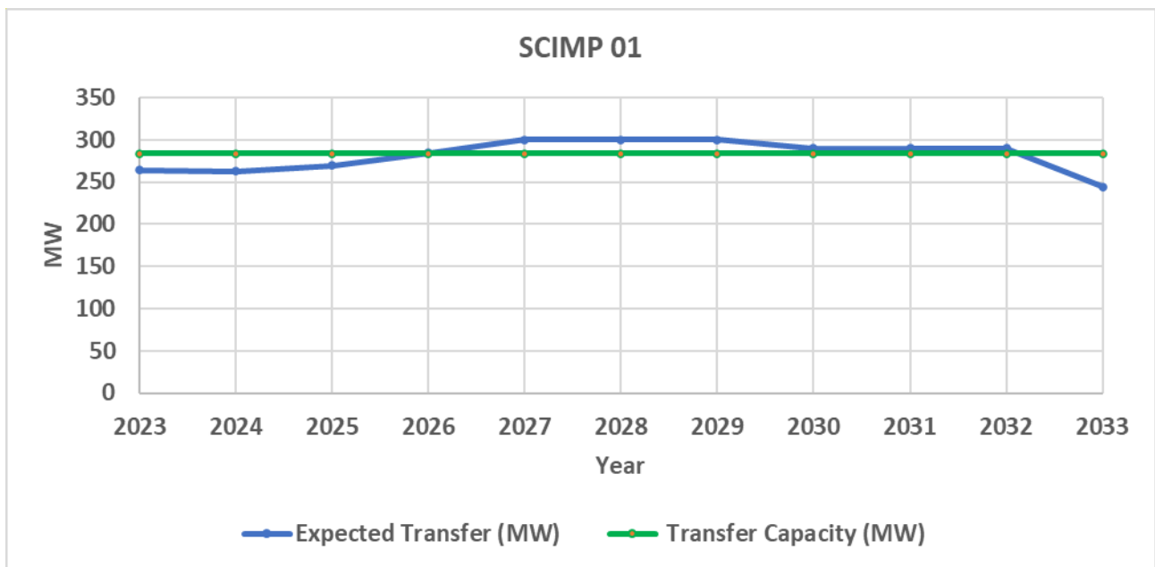
Figure 31: Expected transfer and transfer capacity in SCIMP 01 boundary – peak demand
