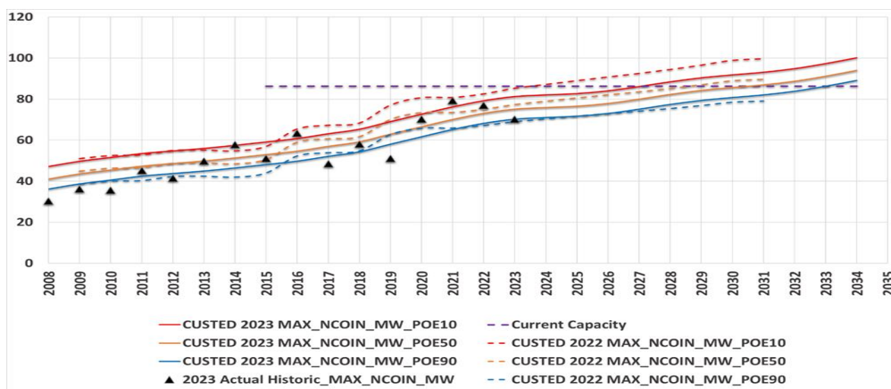
Figure 9: Meadow Springs non-coincidental historical and forecast maximum demand
