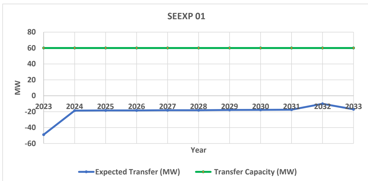
Figure 34: Expected transfer and export transfer capacity in SEEXP 01 boundary – peak demand
