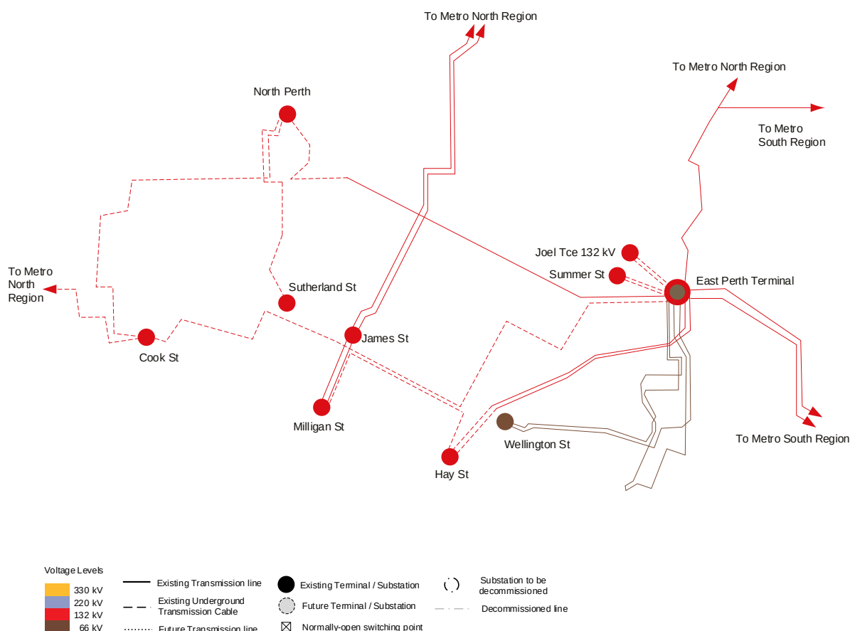
Figure 60: Western Power's East Perth and CBD Region – Network Diagram
