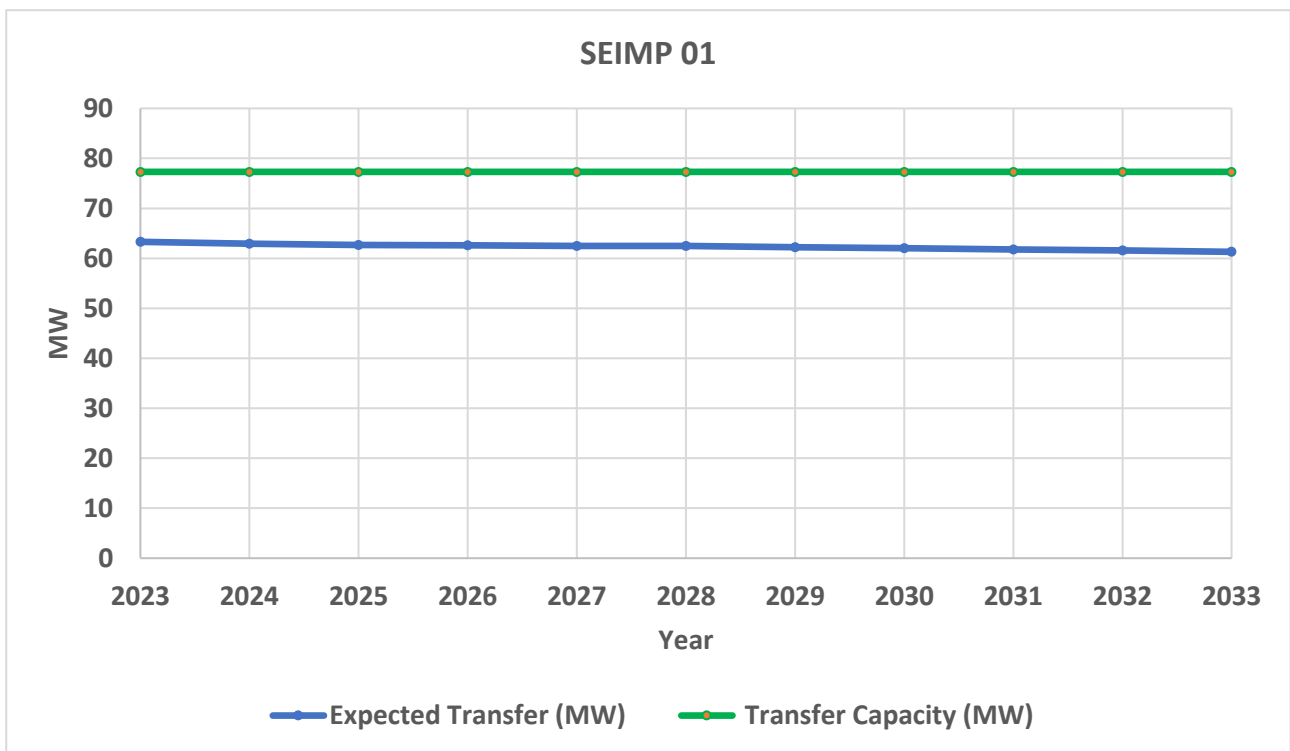
Figure 30: Expected transfer and transfer capacity in SEIMP 01 boundary – peak demand
