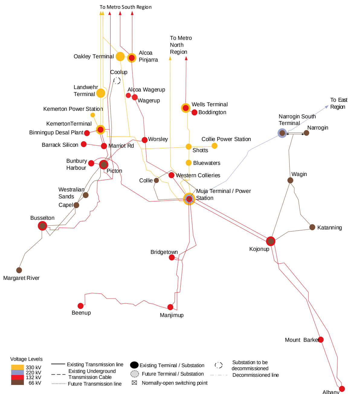
Figure 26: Western Power's South Region – Network Diagram
