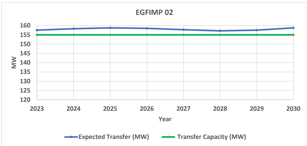
Figure 39: Expected transfer and transfer capacity in EGFIMP 02 boundary – peak demand
