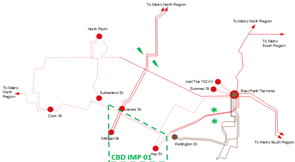
Figure 61: Network import boundaries in the East Perth and CBD Region
