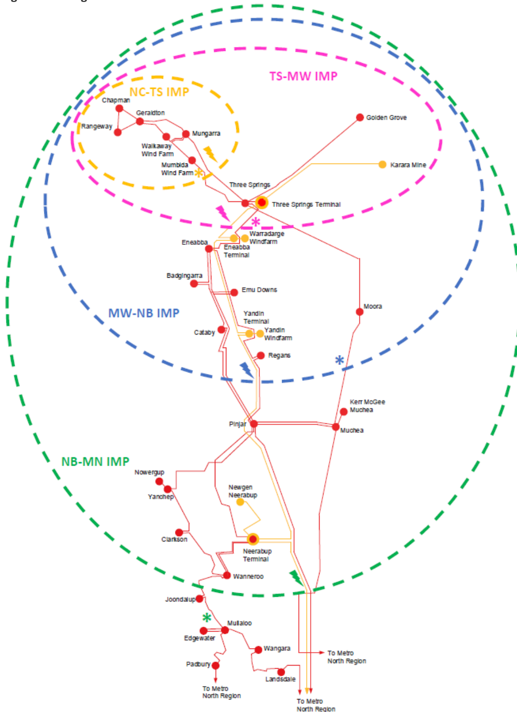
Figure 15: Network thermal import boundaries in the North Region
