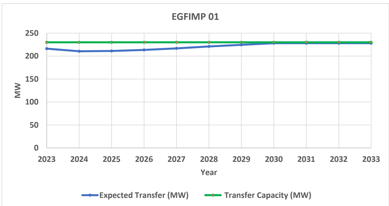
Figure 38: Expected transfer and transfer capacity in EGFIMP 01 boundary – peak demand
