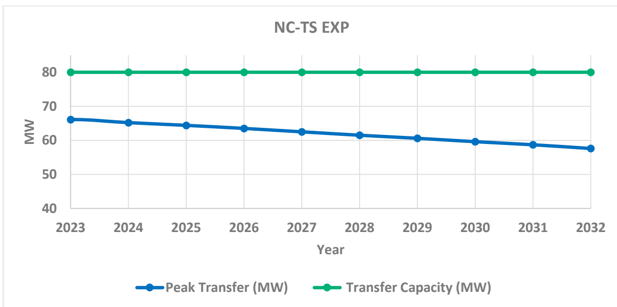
Figure 21: Expected transfer and transfer capacity in NC-TS EXP boundary – peak demand
