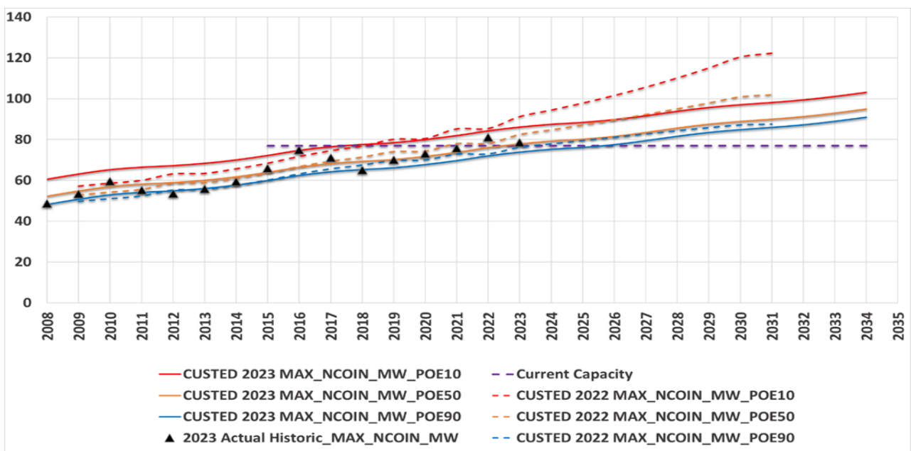
Figure 7: Byford non-coincidental historical and forecast maximum demand
