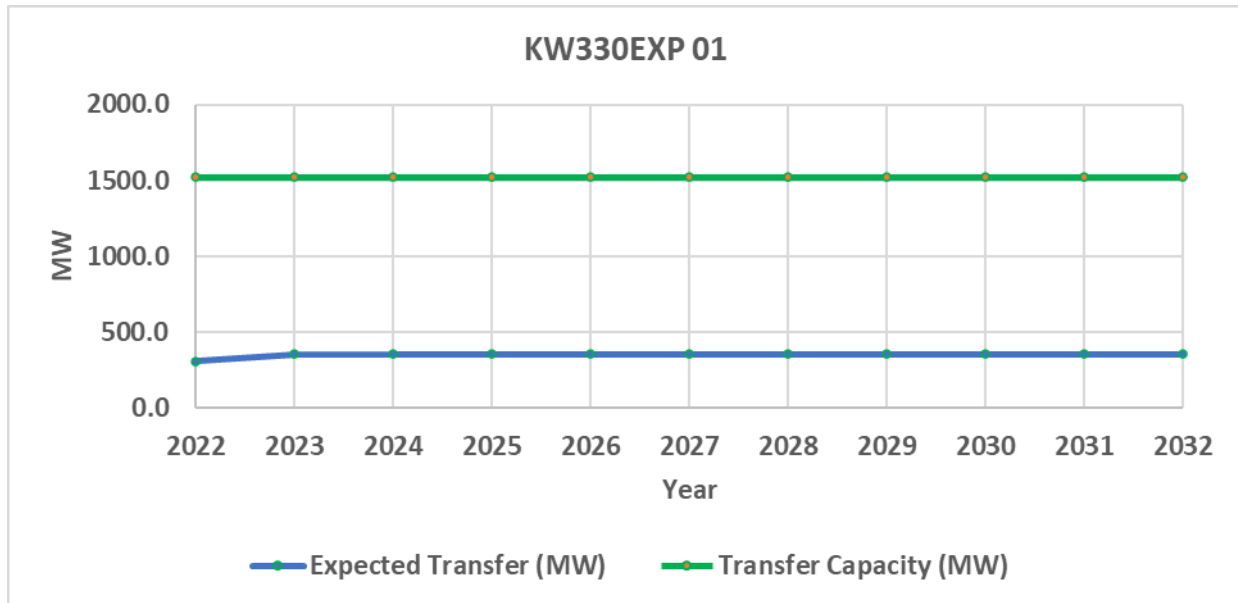
Figure 58: Expected transformer and transfer capacity in KW330EXP 01 boundary – peak demand
