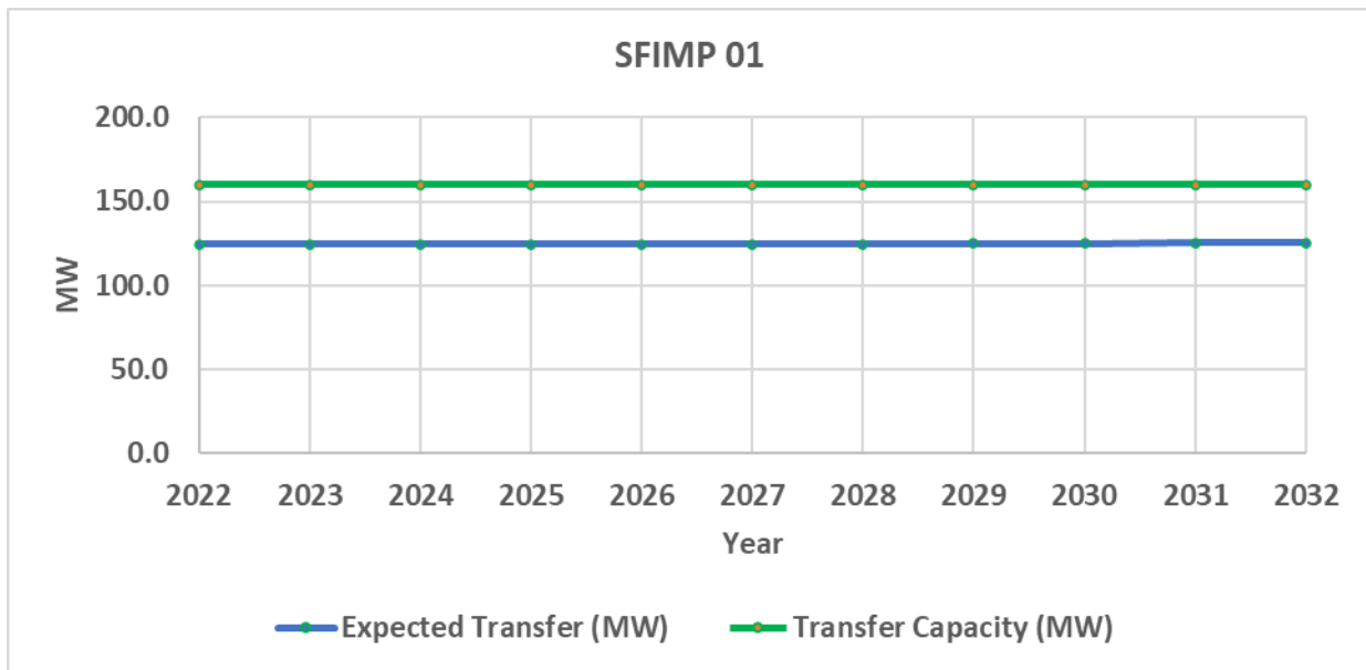
Figure 55: Expected transfer and transfer capacity in SFIMP 01 boundary – peak demand
