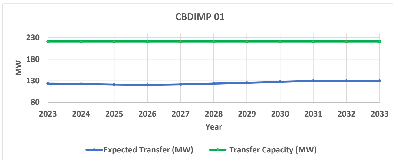
Figure 62: Expected transfer and transfer capacity in CBDIMP 01 boundary – peak demand
