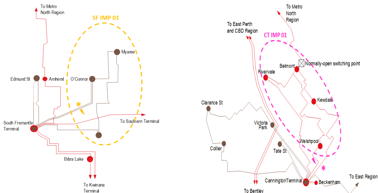
Figure 52: Network import boundaries in the Metro South Region – South Fremantle and Cannington
