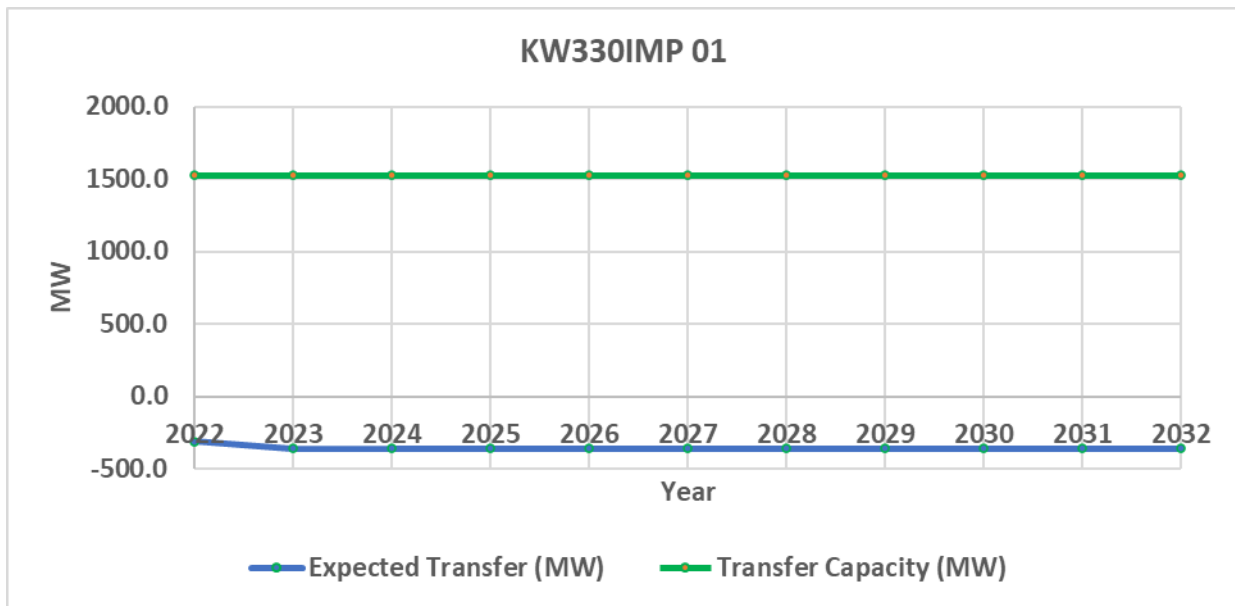
Figure 53: Expected transfer and transfer capacity in KW330IMP 01 boundary – peak demand
