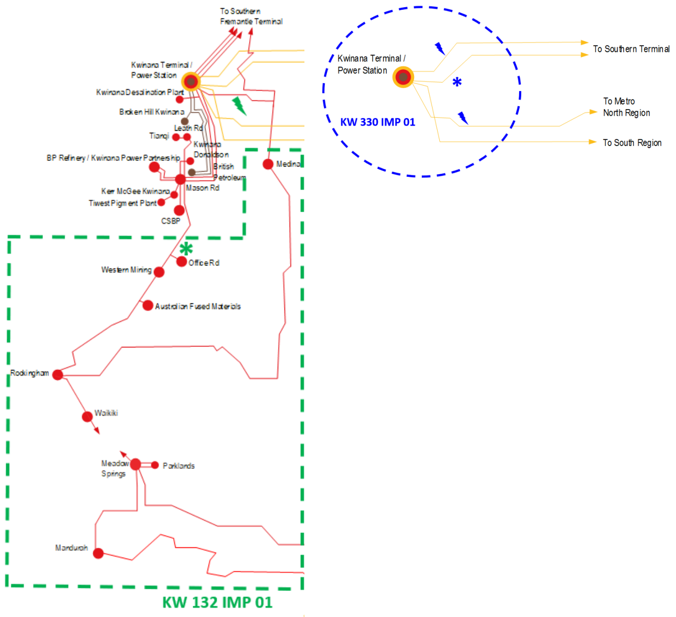
Figure 51: Network import boundaries in the Metro South Region – Kwinana 330 kV and 132 kV
