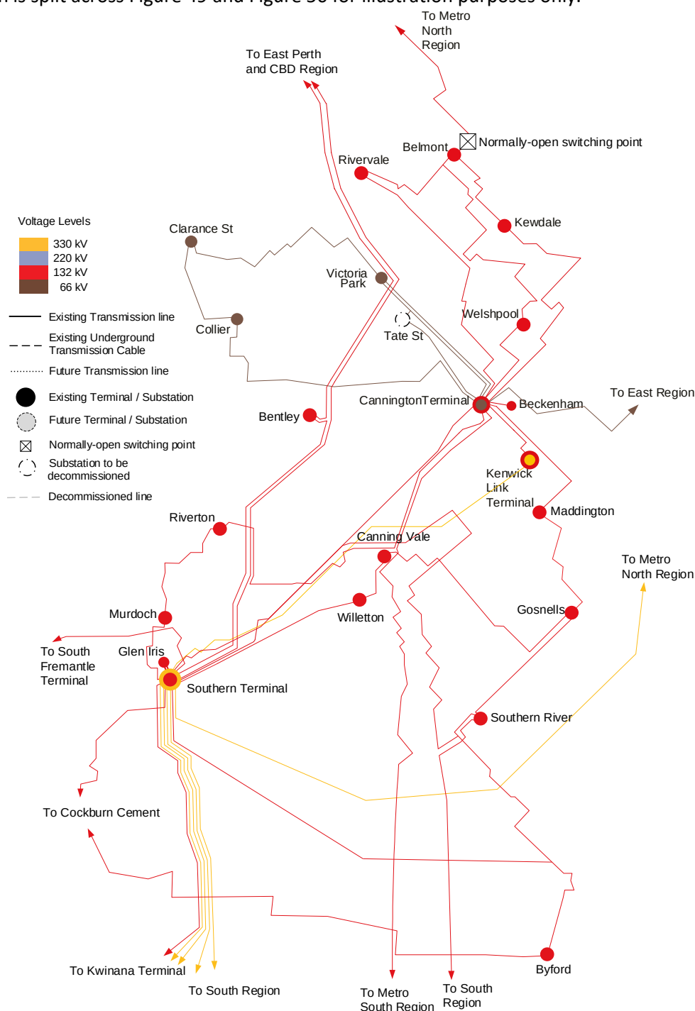
Figure 49: Western Power's Metro South Region (Part A) – Network Diagram
