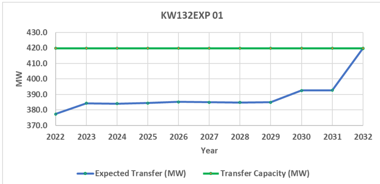
Figure 59: Expected transfer and transfer capacity in KW132EXP 01 boundary – peak demand
