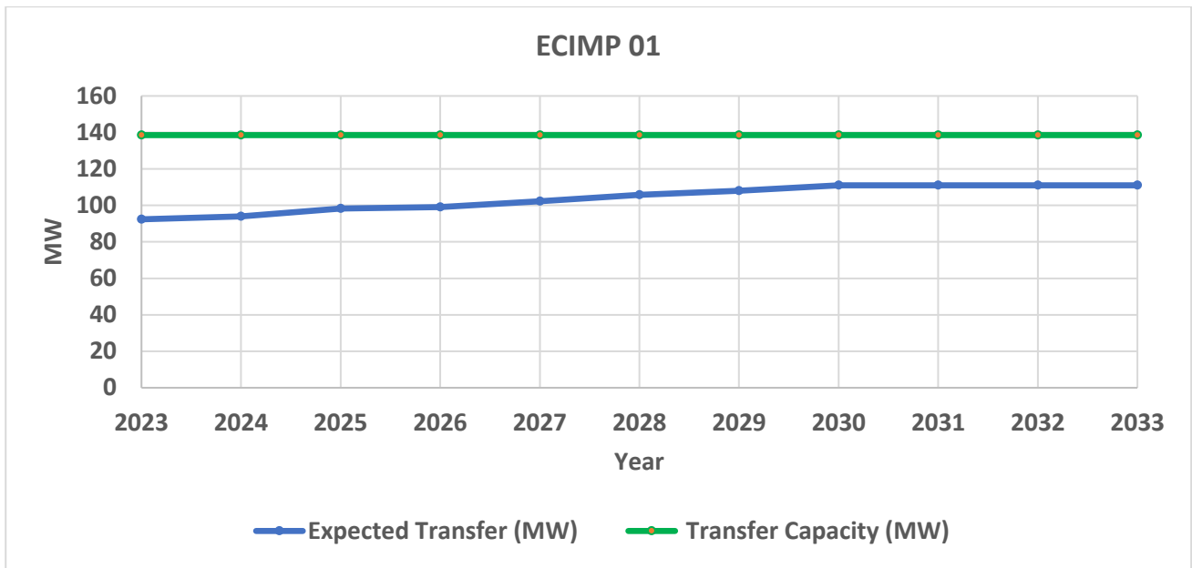
Figure 37: Expected transfer and transfer capacity in ECIMP 01 boundary – peak demand
