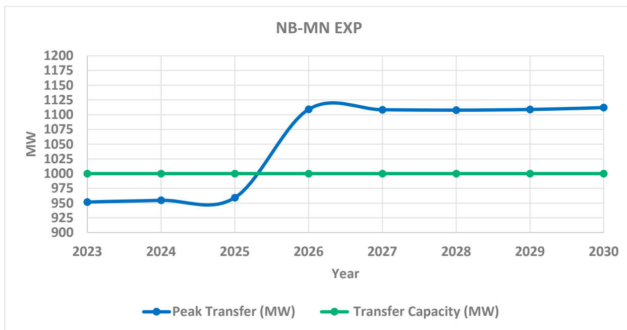
Figure 24: Expected transfer and transfer capacity in NB-MN EXP boundary – peak demand
