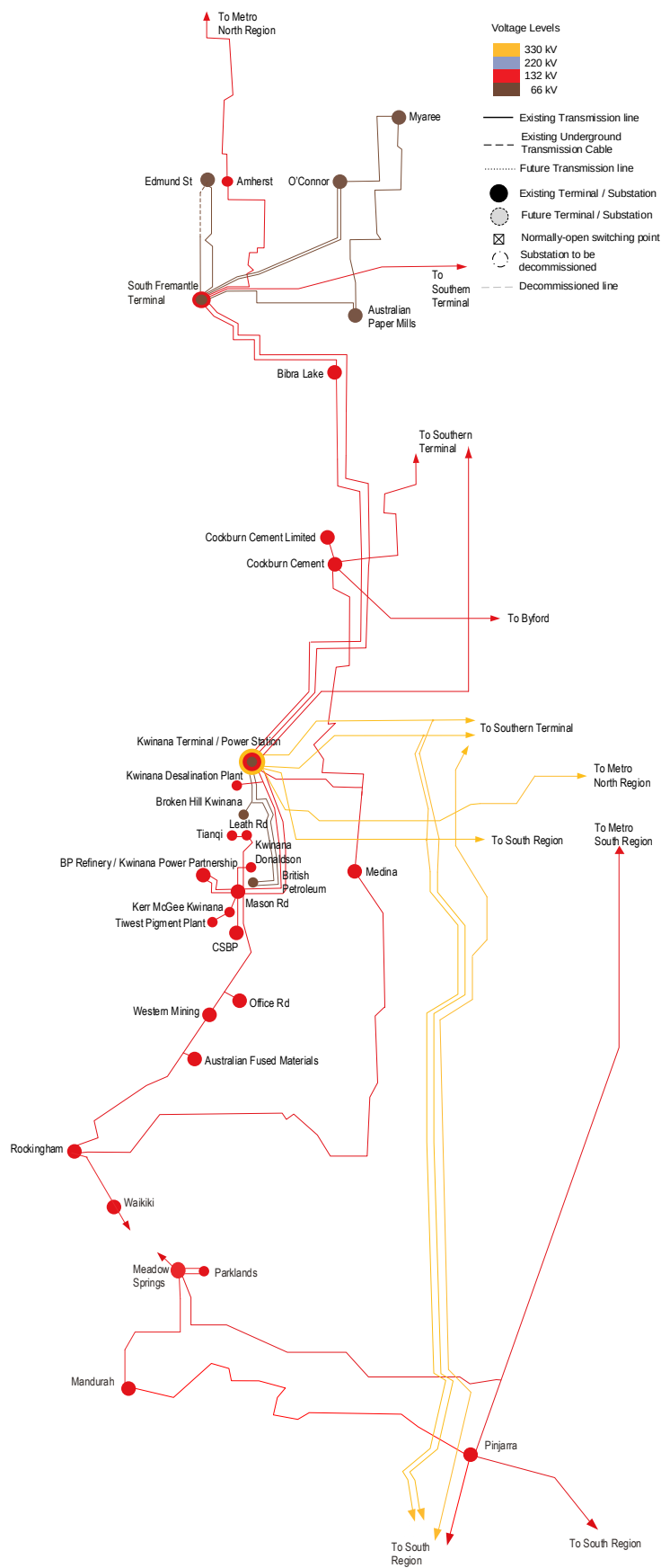
Figure 50: Western Power's Metro South Region (Part B) – Network Diagram
