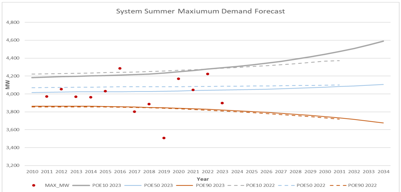
Figure 6: Historical and forecast system maximum demand – 2022 and 2023
