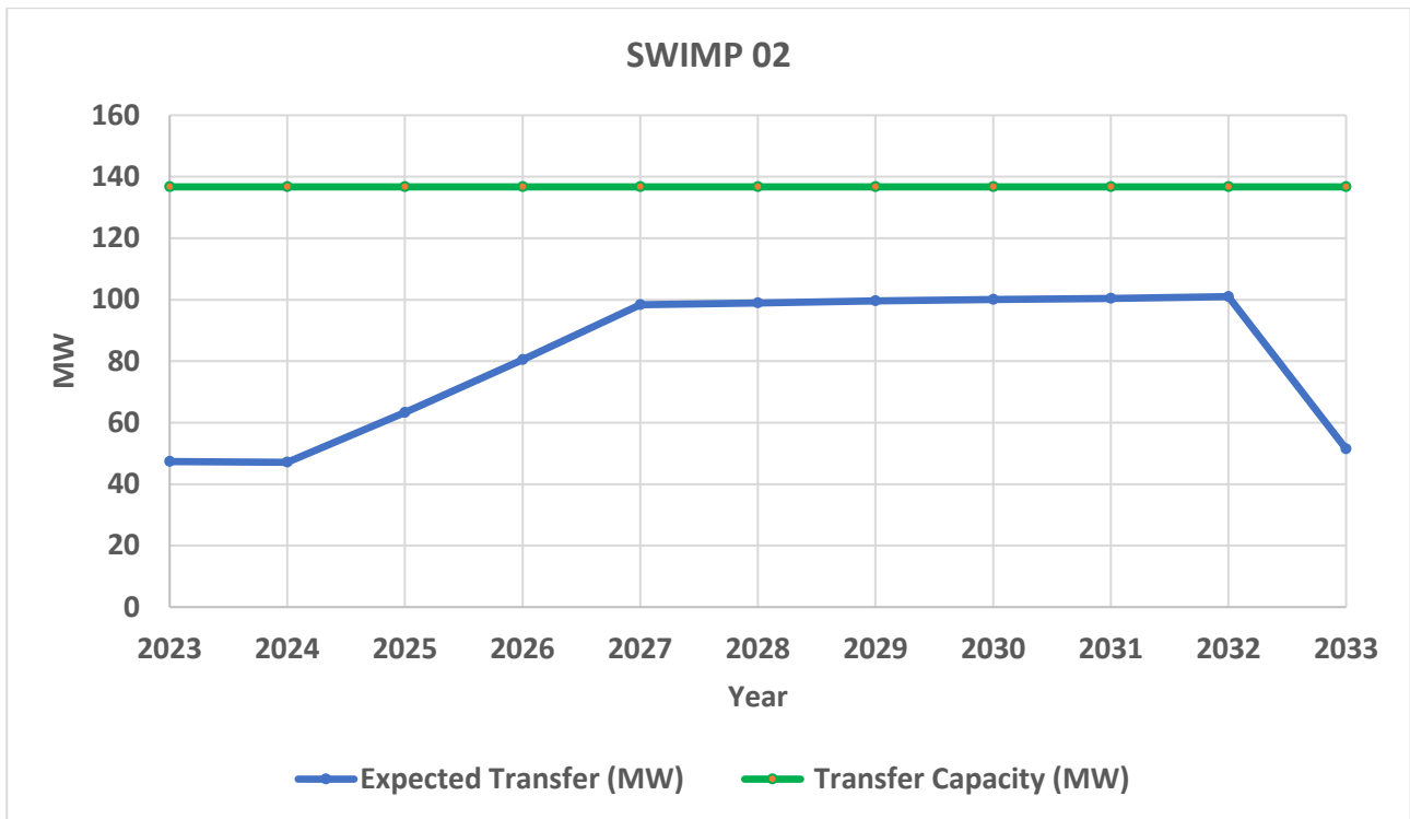
Figure 29: Expected transfer and transfer capacity in SWIMP 02 boundary – peak demand
