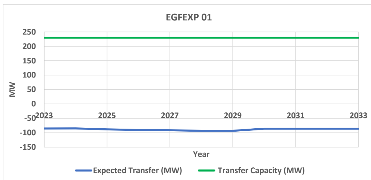
Figure 42: Expected transfer and transfer capacity in EGFEXP 01 boundary – peak demand
