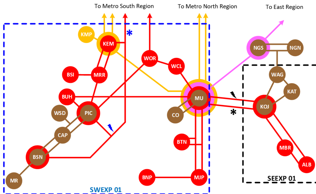
Figure 32: Network export boundaries in the South Region
