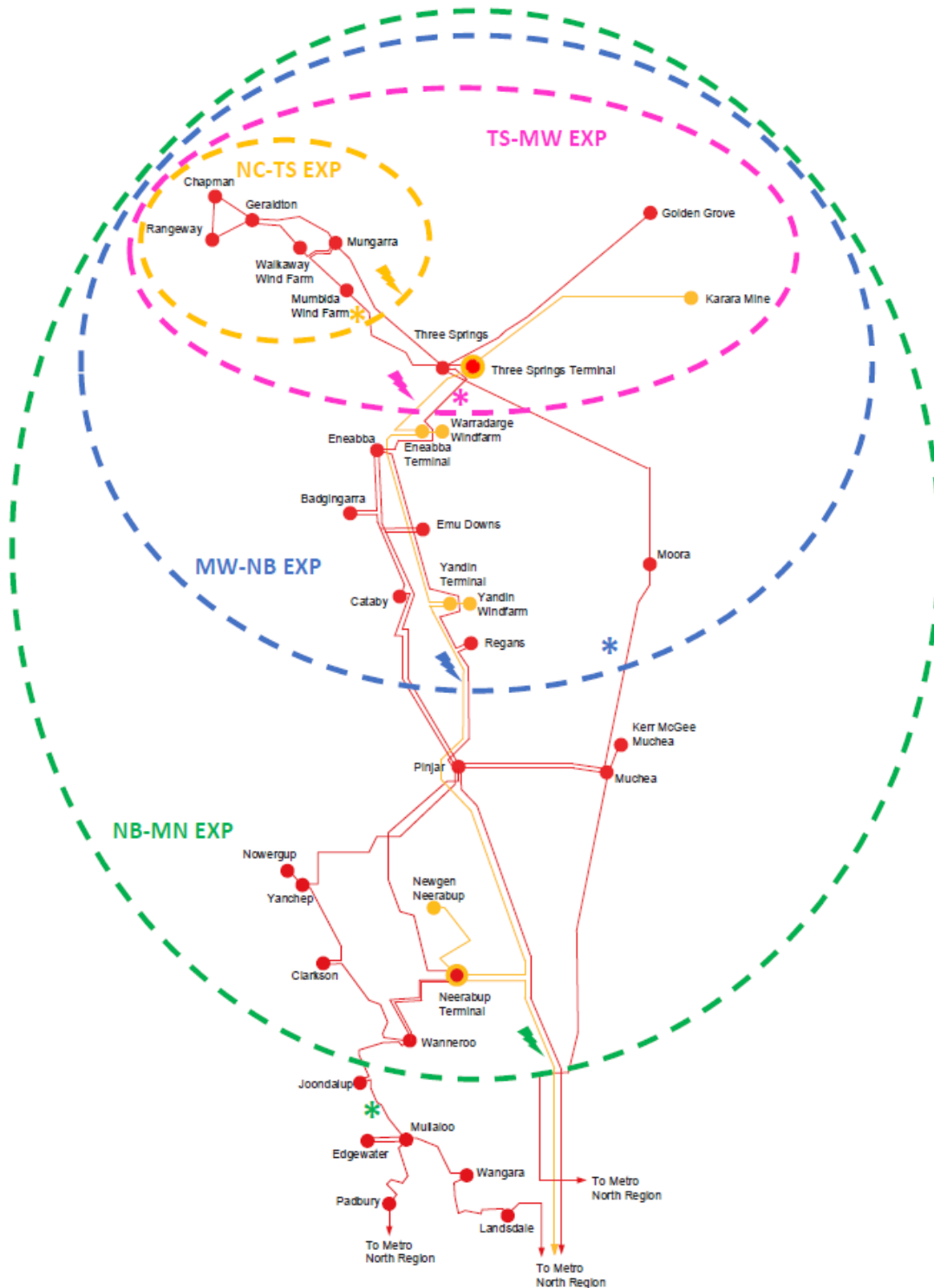
Figure 20: Network thermal export boundaries in the North Region
