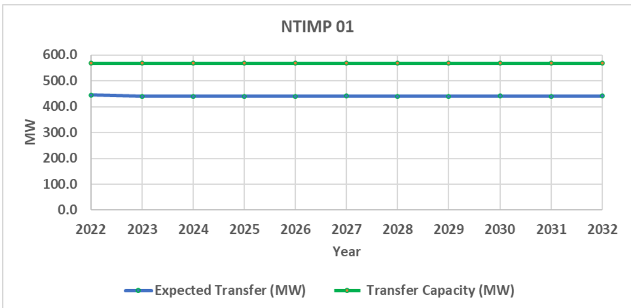
Figure 47: Expected transfer and transfer capacity in NTIMP 01 boundary – peak demand
