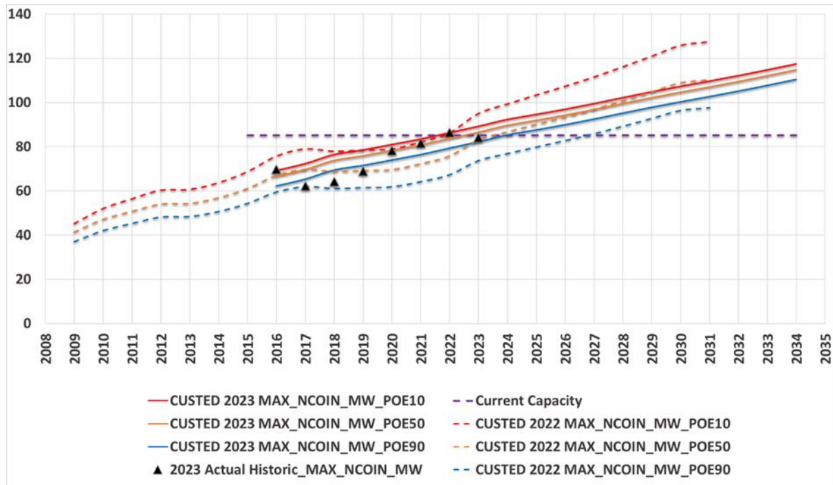
Figure 10: Southern River non-coincidental historical and forecast maximum demand
