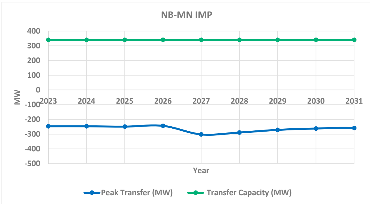
Figure 19: Expected transfer and transfer capacity in NB-MN IMP boundary – peak demand
