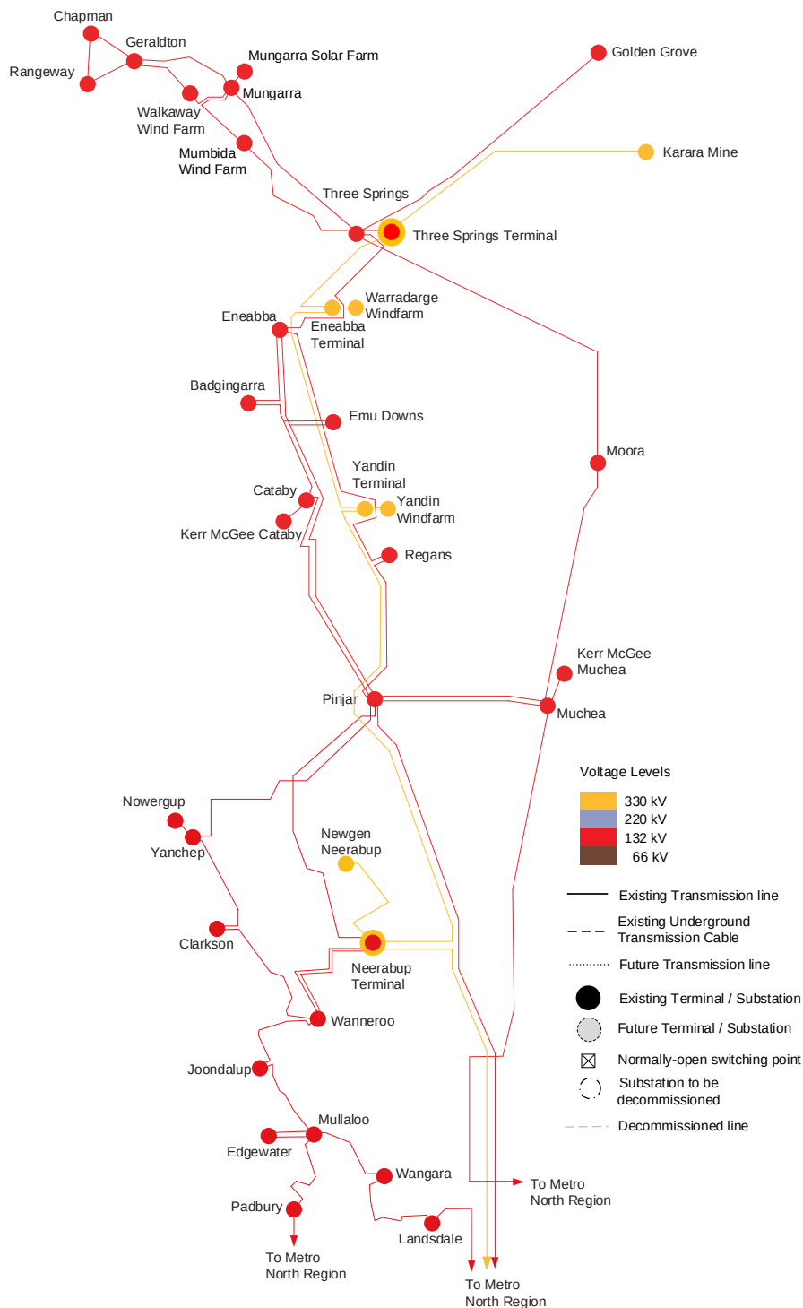
Figure 14: Western Power's North Region – Network Diagram
