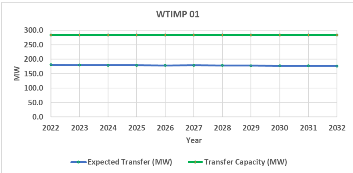
Figure 46: Expected transfer and transfer capacity in WTIMP 01 boundary – peak demand
