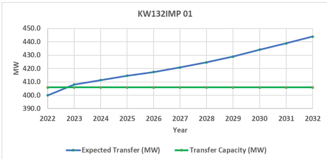
Figure 54: Expected transfer and transfer capacity in KW132IMP 01 boundary – peak demand
